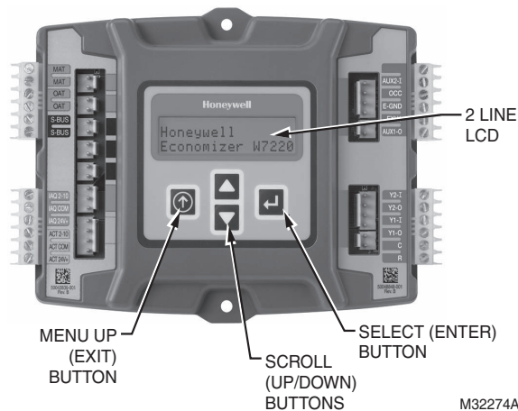
Fig. 11. Economizer LCD and Keypad Layout.
