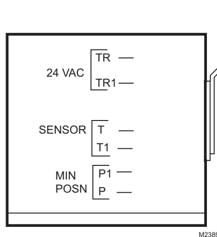
M7415 modulating motor, sensor input or controller required. Used with W7459A or D only.
