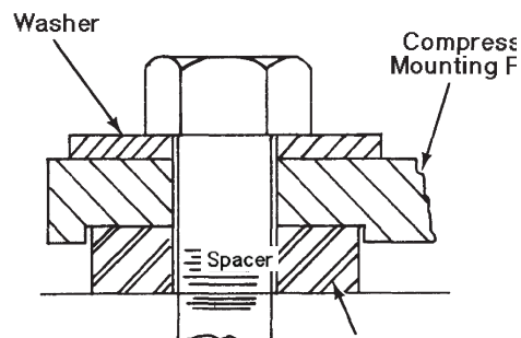
Solid Mount for Mobile or Deep Sump Application
