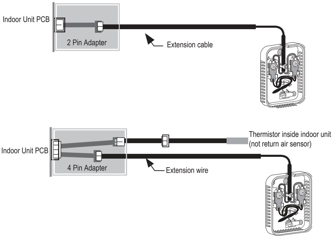
Connection Example (refer to installation manual for complete details)
