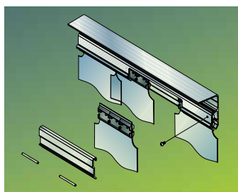
Maximum duty system made of heavy gauge aluminum extrusions to carry heavy loads and last.
